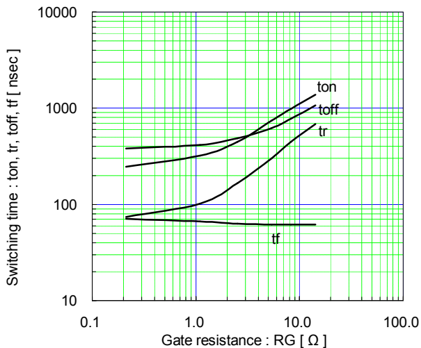
Switching time vs. Gate resistance (typ.) V_{cc}=600V, I_c=450A, V_{GE}=\pm 15V, T_j=25^\circ C
